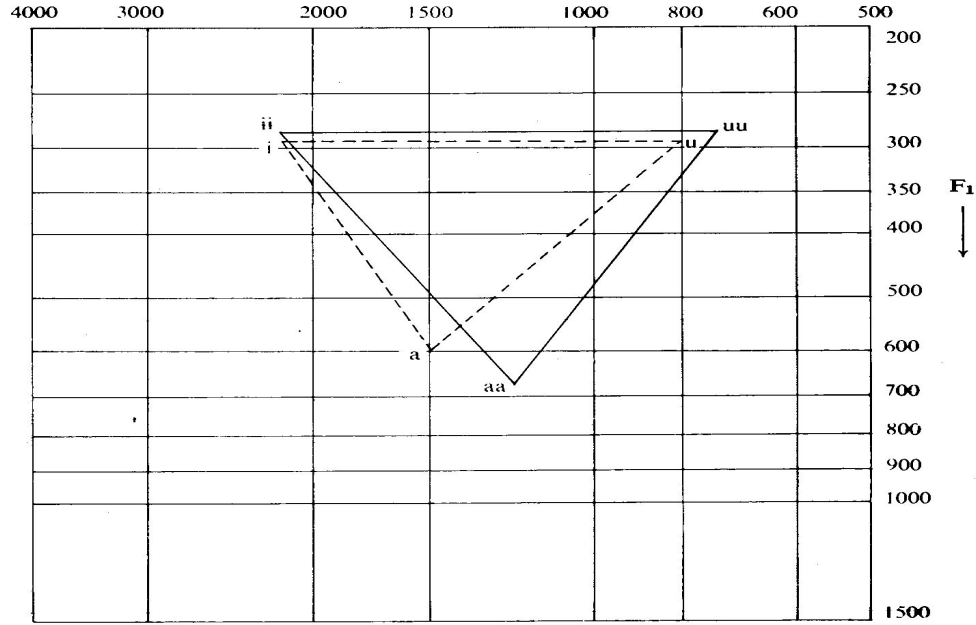
DIAGRAM I Short and Long Vowels in Isolation ← F 2 F 1 ↓
